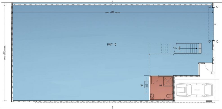
WAREHOUSE 10 PLAN SCALE: 1/8" = 1'-0"
